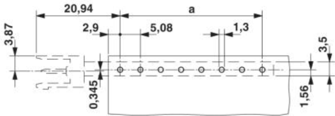
Dimensional drawing
